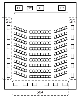
Multiple surround speakers (For 6.1-channel system)
